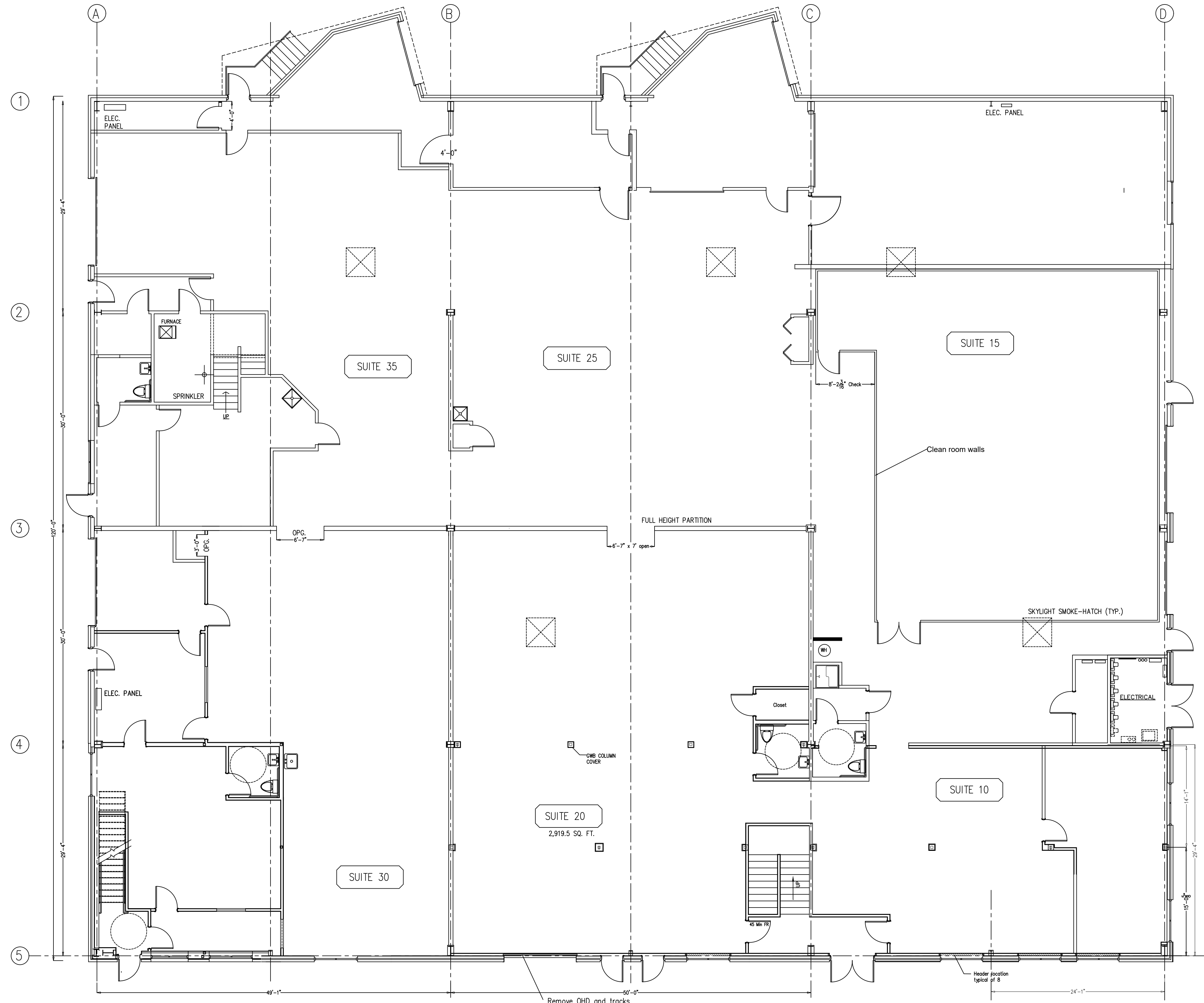
1st FLOOR FINAL LAYOUT 05-22-19
