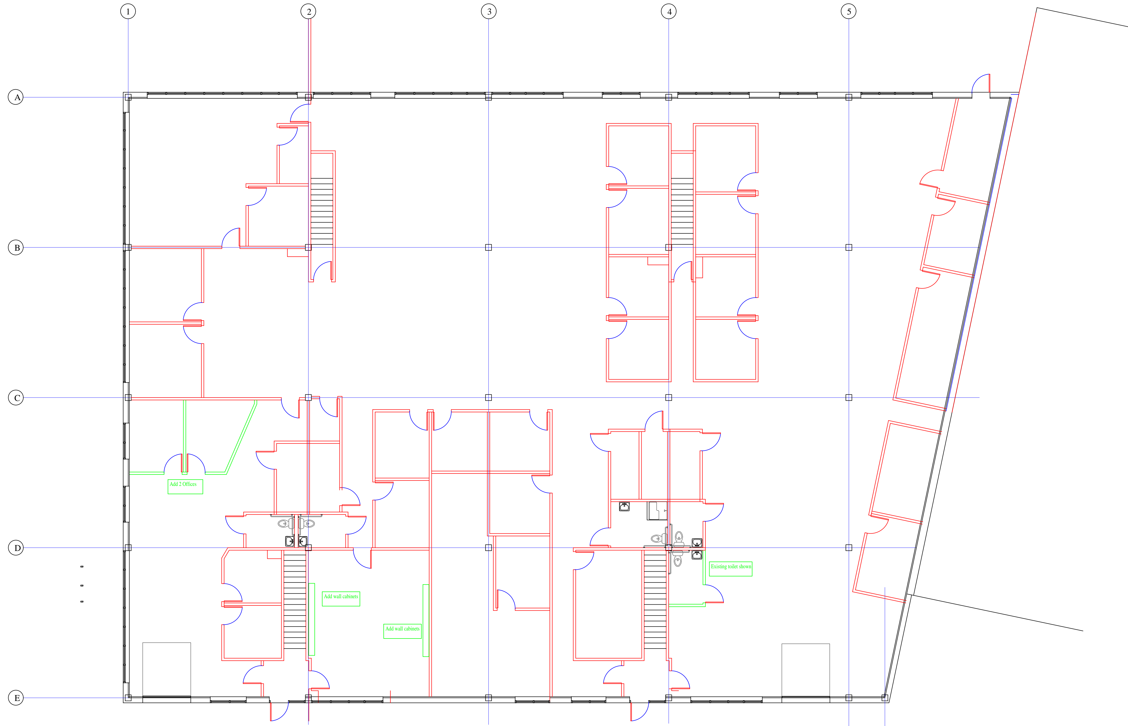
UPPER LEVEL FLOOR PLAN SCALE: 1/8" = 1'-0"
